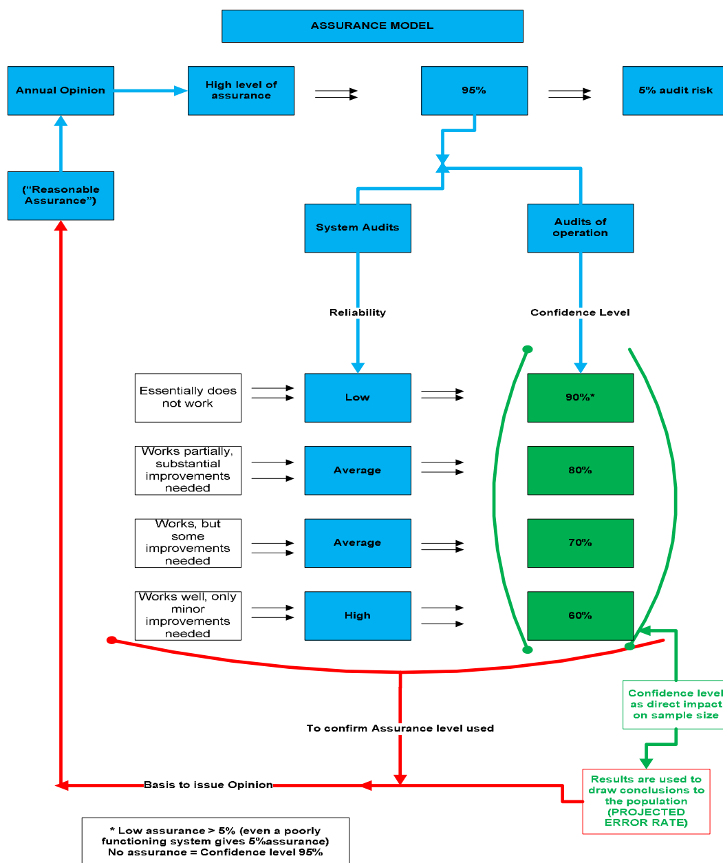
Figura 15: Assurance model
