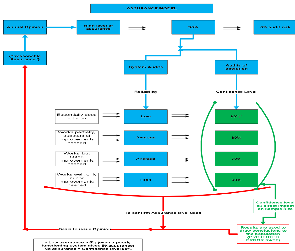
Figura 11: Assurance model
